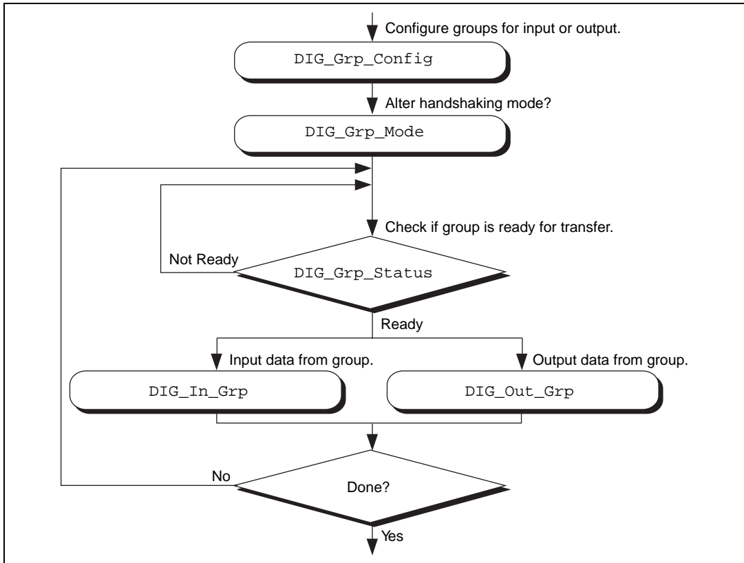
Figure 3-23. Simple Digital Group Input or Output Application
