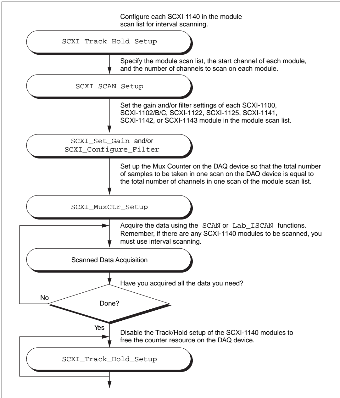
Figure 3-43. Channel-Scanning Operation Using Modules in Multiplexed Mode
