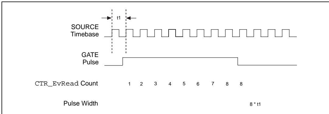
Figure 3-32. Pulse Width Measurement
